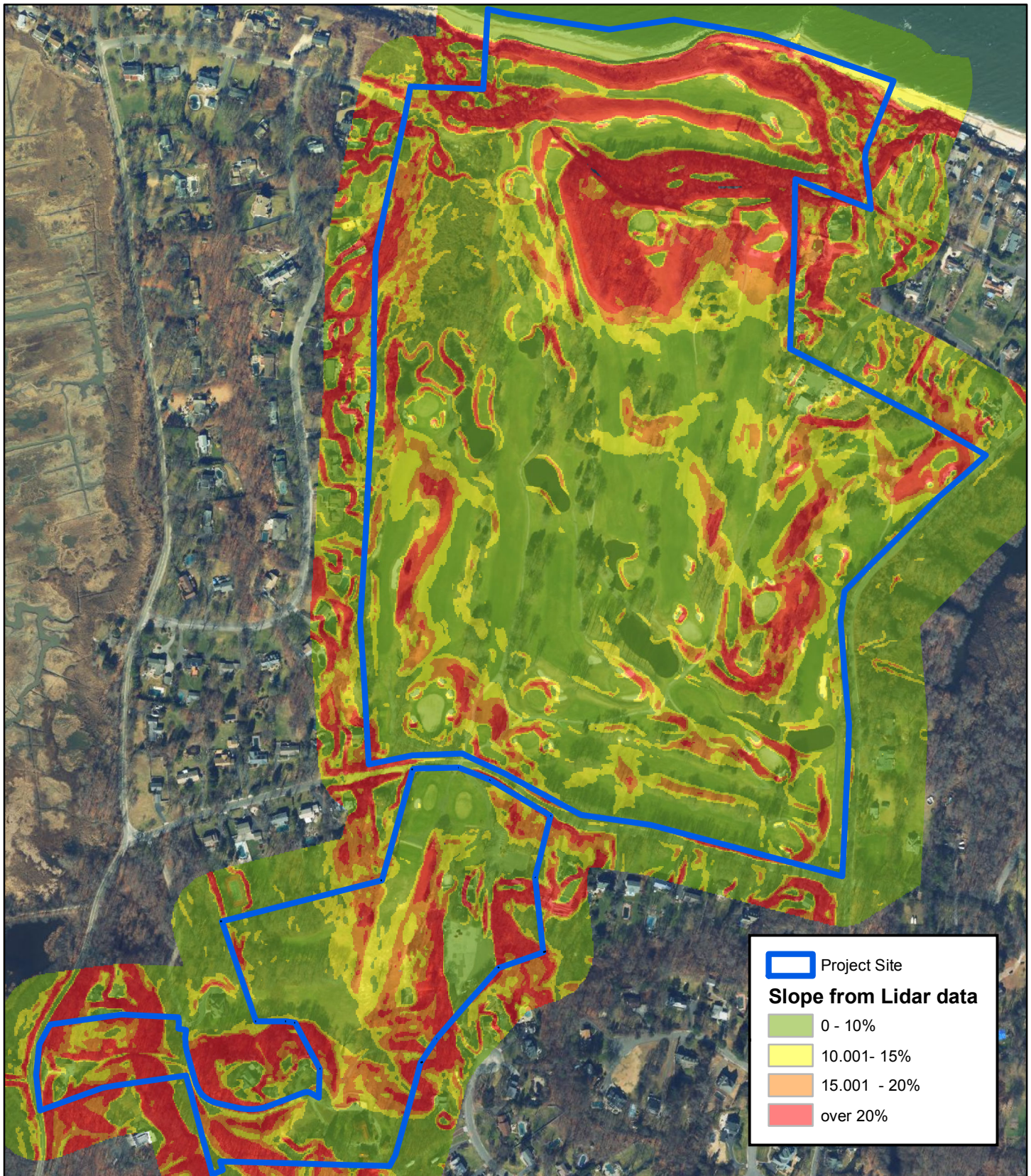
FIGURE 2-2 SLOPES
